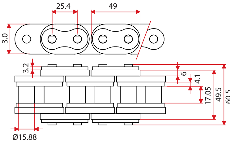
5118.000.09 Sharp top chain 16B-1
