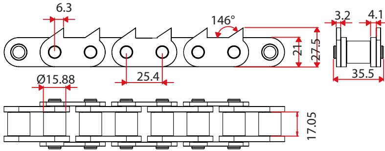
5118.000.51 Sharp top chain 16B-1
