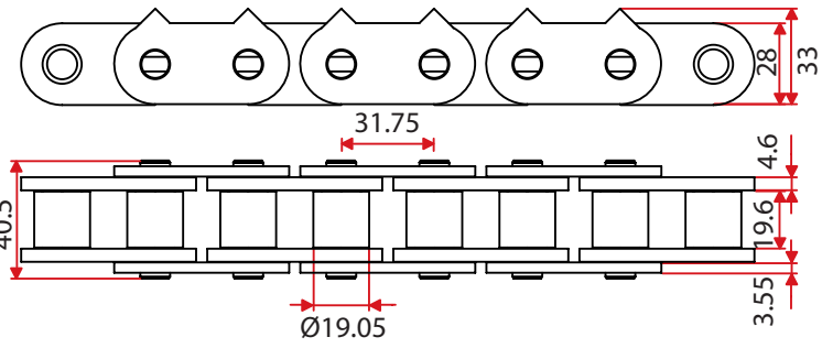
Sharp top chain 20B-1
