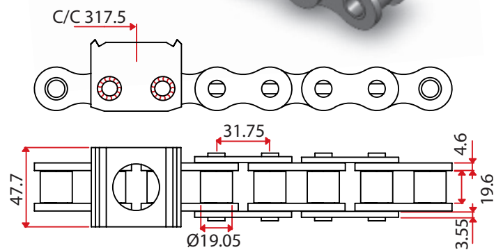
Sharp top chain 20B-1
