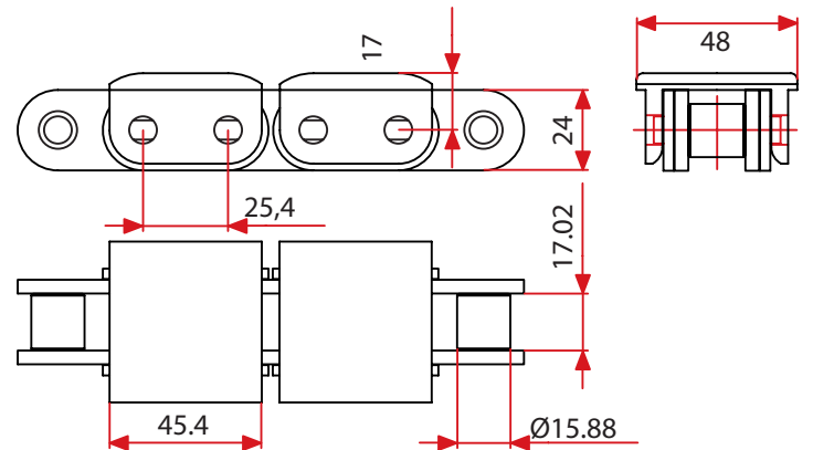
5212.000.08 Sharp top chain with plastic cover. 16B-1
