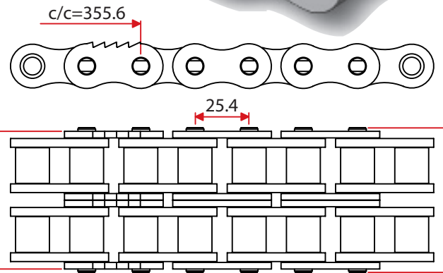
5218.000.20 Sharp top chain 16B-2
