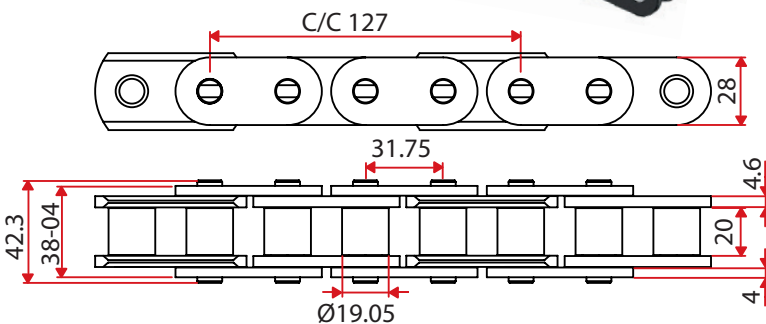
Sharp top chain 20B-1
